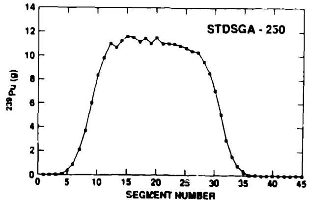
Fig. 3. Vertical scan of the standard STDSGA-250.
