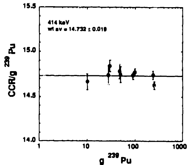
Fig. 5. Measurements for set A of the standards plus one of the measurement control standards (STDGMC-6).
